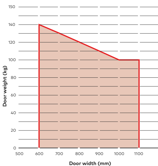
Max. permissible door widths and weights
